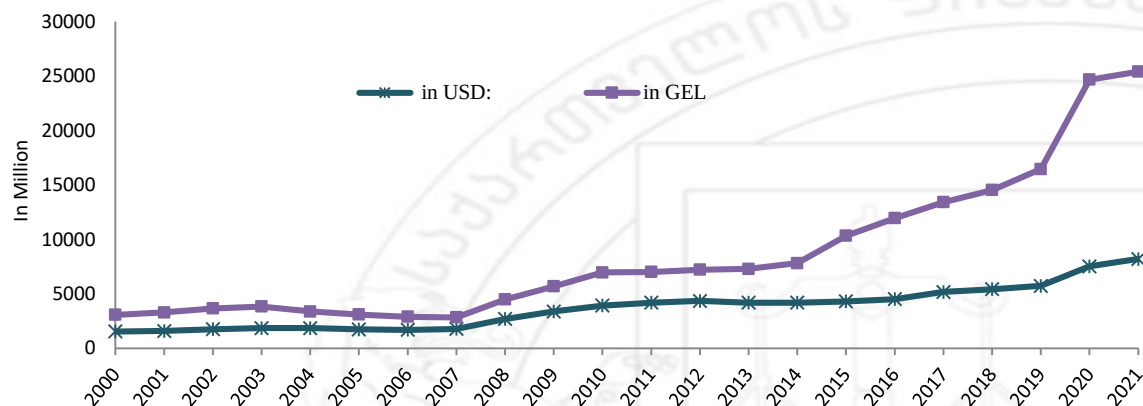
4. EXTERNAL PUBLIC DEBT OF GEORGIA
